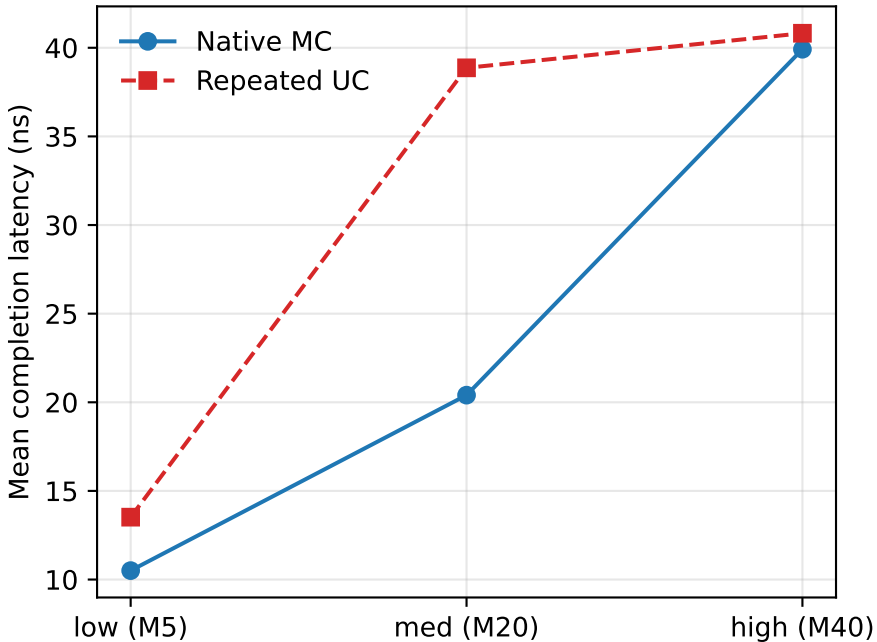
Fig.256-2a Completion latency (tick=1)
