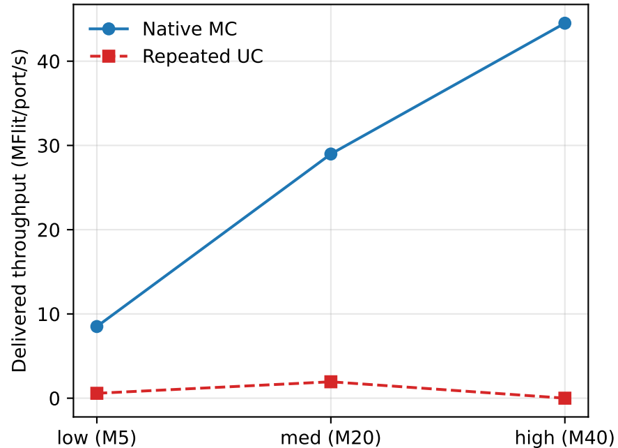
Fig.256-2b Useful delivery throughput
